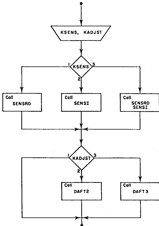
Fig. 1. ALVIN structure.
